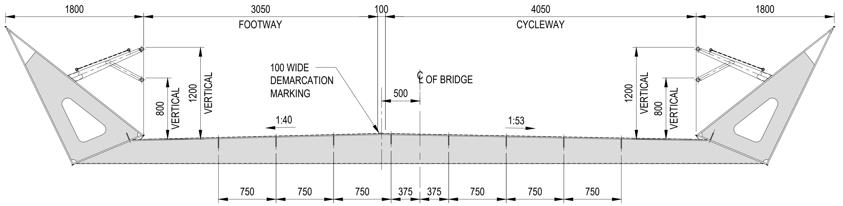
TYPICAL CROSS SECTION ( ii ) (TAKEN AT MID CENTRAL SPAN - SHOWING 'WING UP' CONDITION)
